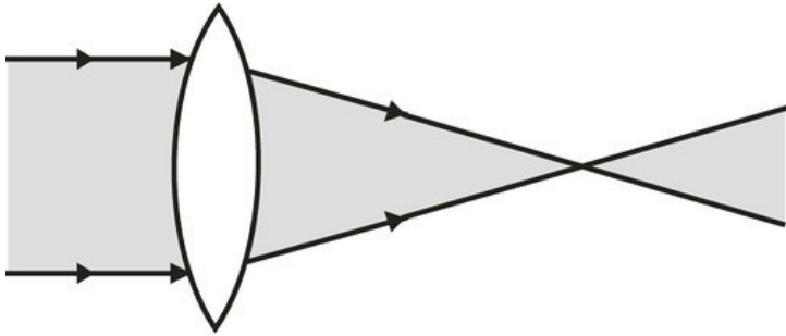
Convex lens
