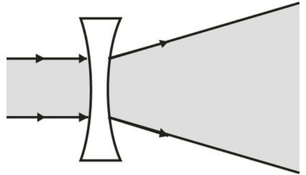
Concave lens
